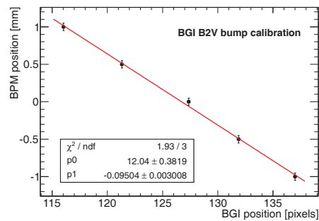
Figure 5: Calibration of the BGI scale using orbital bump.
