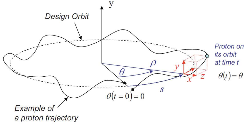
Figure 2.2: Sketch of a proton on a trajectory different from the design orbit [12].
