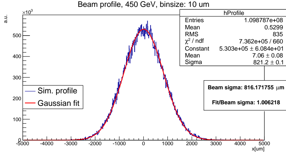
Figure 4.1: Profile of 450 GeV beam obtained by tracking the liberated electrons (histogram) and a Gaussian fit.
